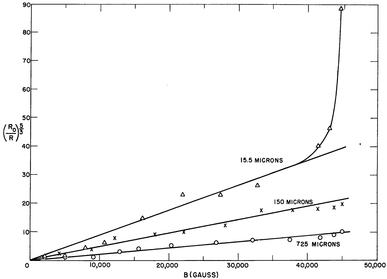
Fig. 13 Plots of (\frac{R_0}{R})^{5/3} as a function of B for three different values of the initial base deuterium pressure.
