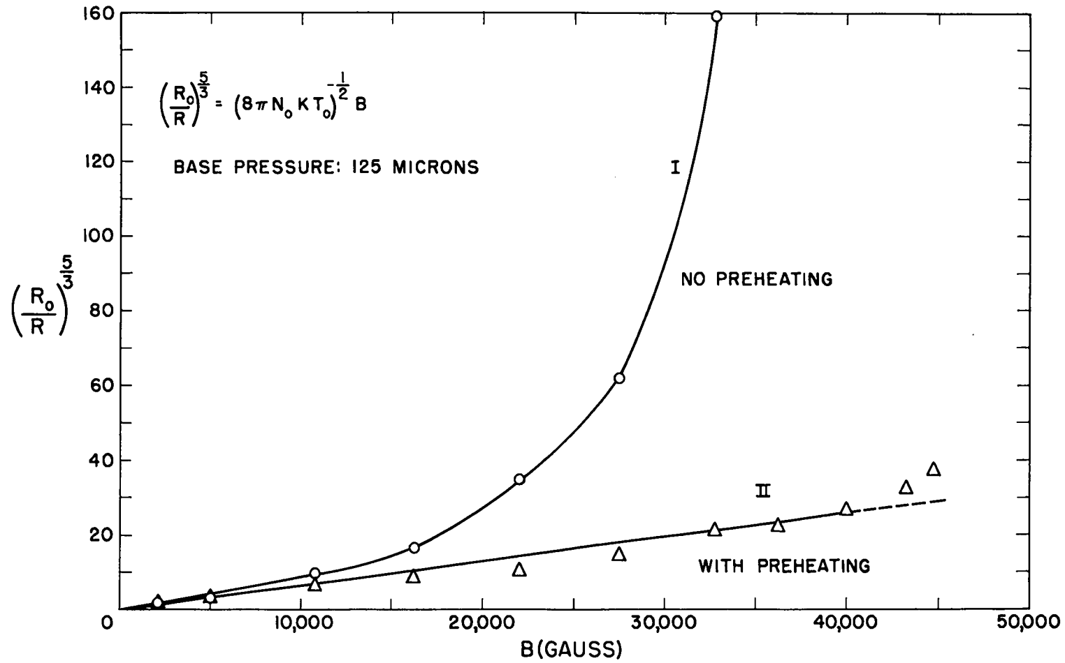
Fig. 12 Plots of (R_0/R)^{5/3} as a function of B without shock preheating (Curve I) and with shock preheating (Curve II). The base pressure of deuterium was 125 microns.
